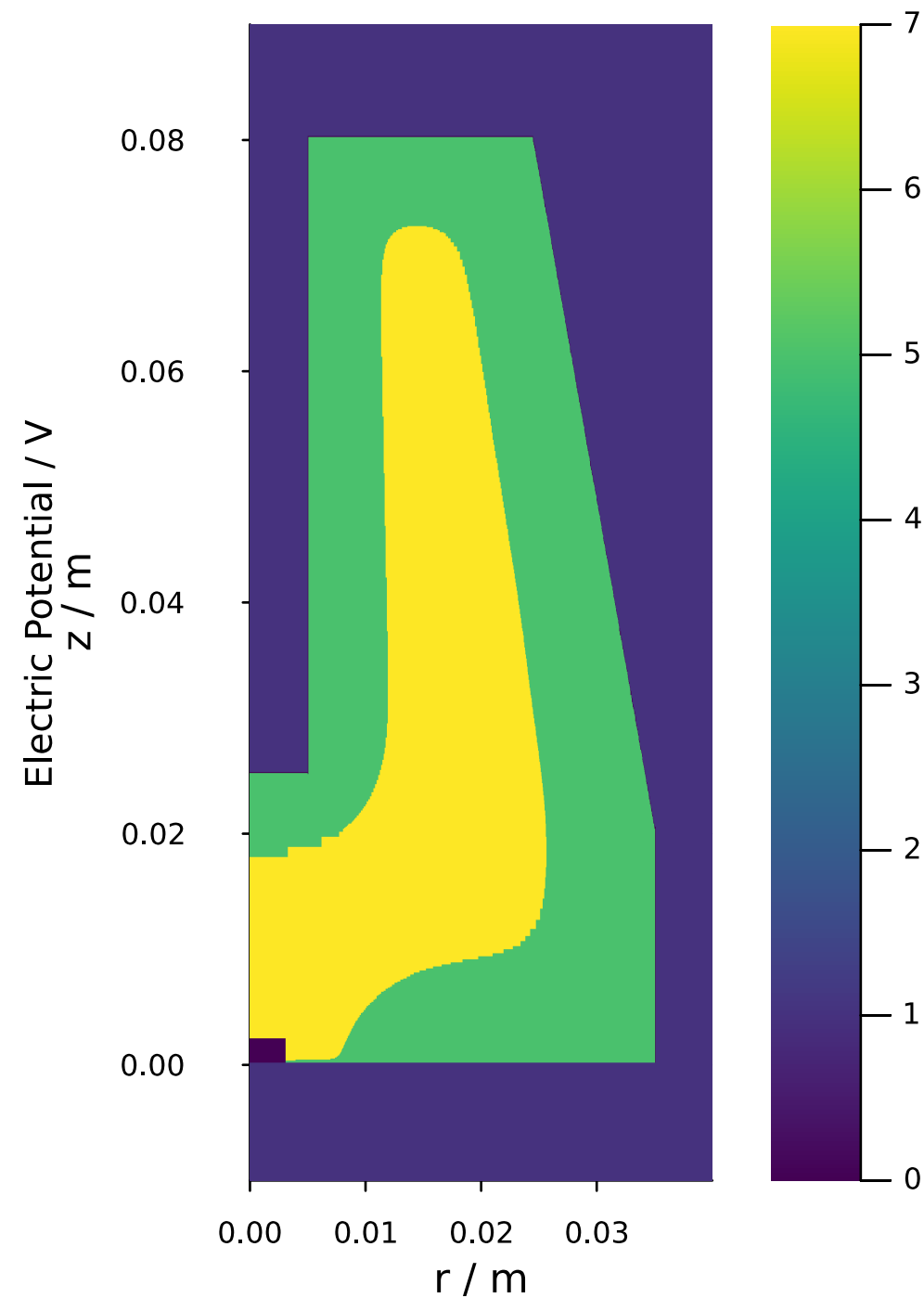
Point Type Map @ \phi = 0.0^\circ
