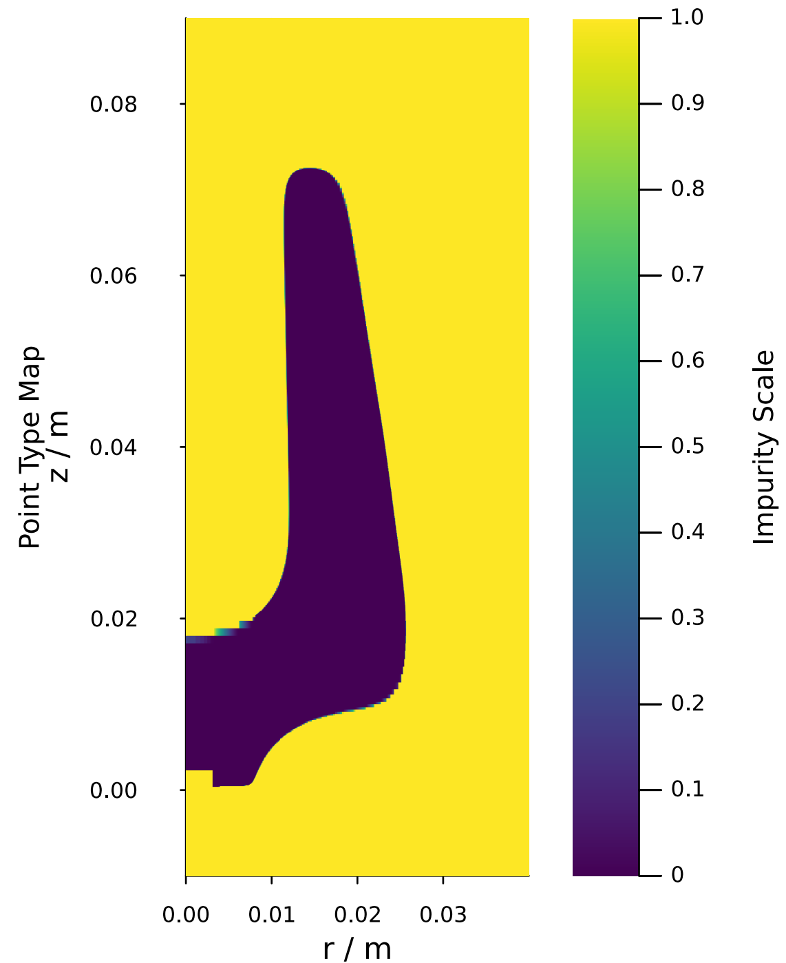
Impurity Scale @ \phi = 0.0^\circ
