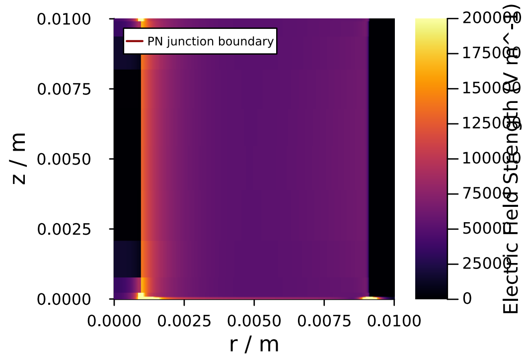
electric field
