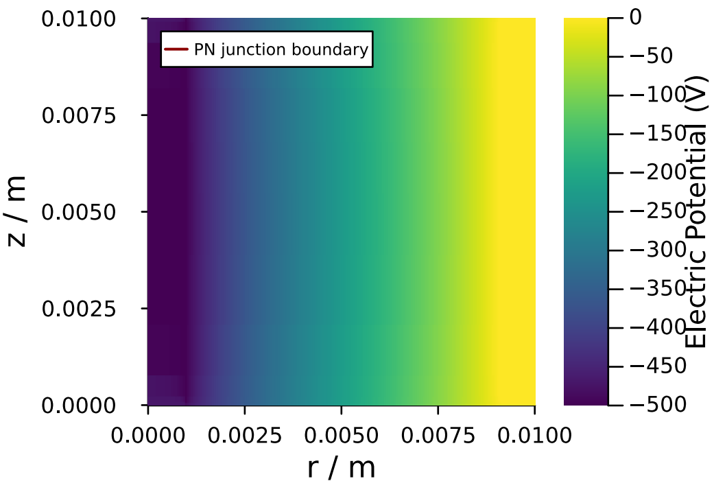
electric potential
